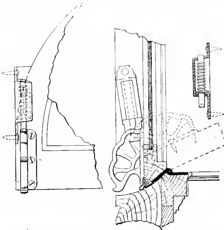
Fig. 4391-4393. Sectional Elevations. PULLMAN DECK-SASH PIVOT AND RATCHET-CATCH.
